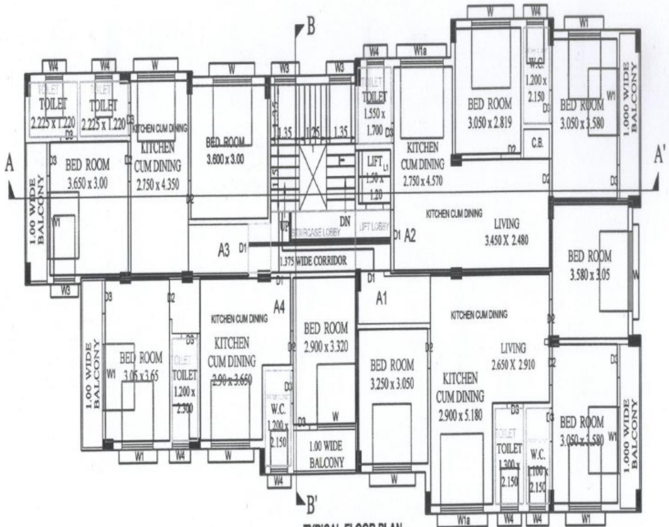
TYPICAL FLOOR PLAN (1ST, 2ND, 3RD. & 4TH.)
